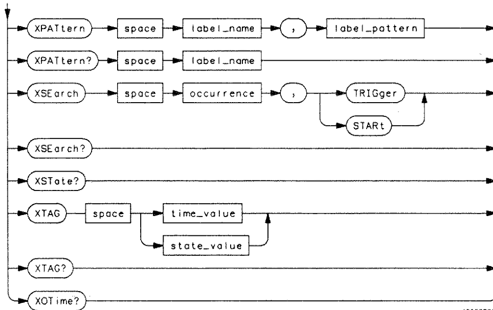
SLISt Subsystem Syntax Diagram (continued)
