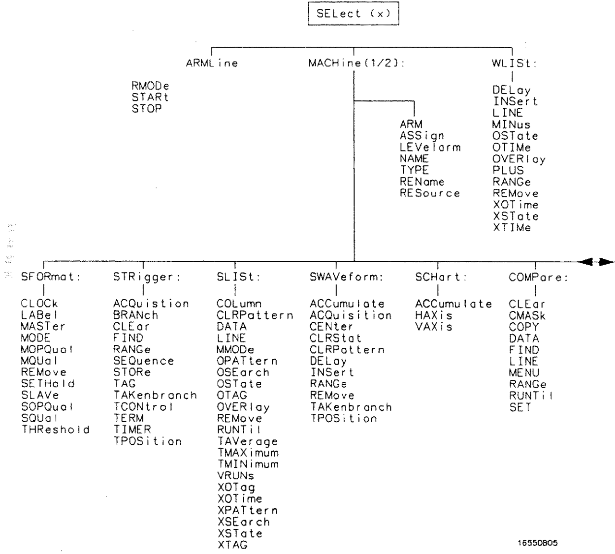
HP 16550A Command Tree
