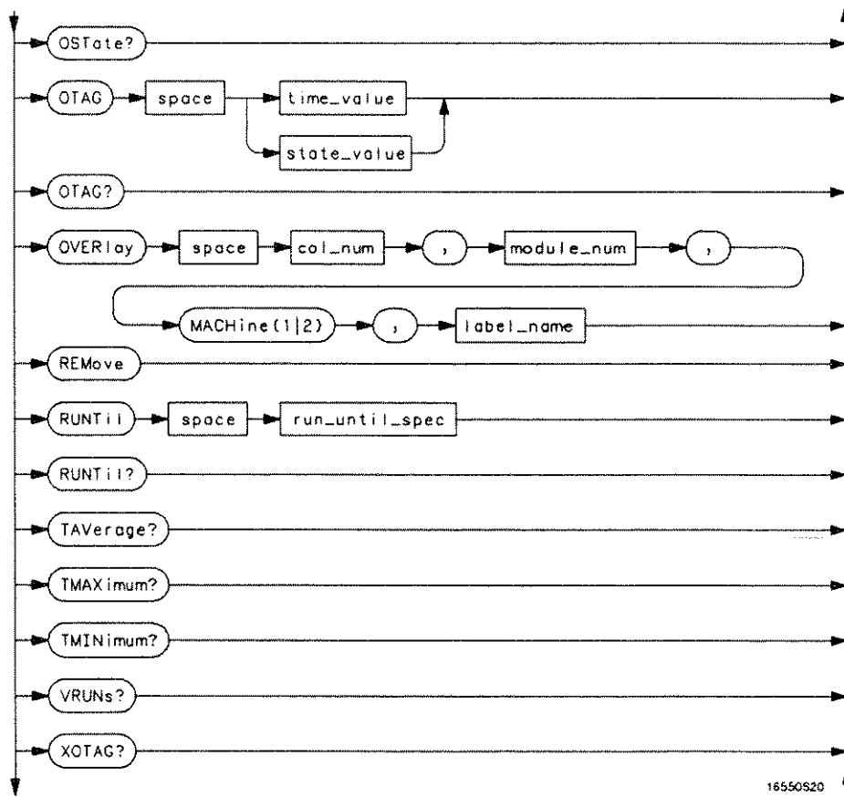
SLISr Subsystem Syntax Diagram (continued)
